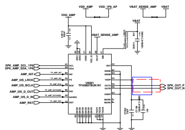
Audio amp
