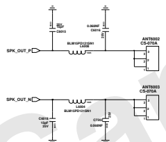
SPK Connector
